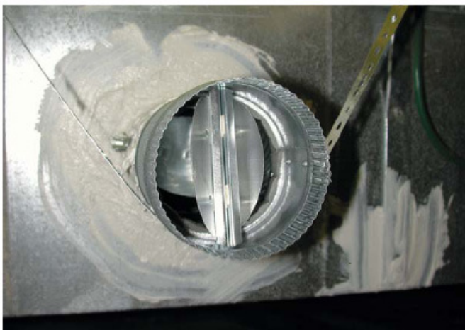
The butterfly damper of this crawlspace supply opens while the system is running. The assembly is sealed with mastic and supported by strapping to ensure that the butterfly damper continues to operate properly.
